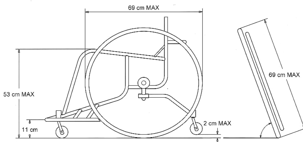
Diagram 5 Wheelchair Dimensions
